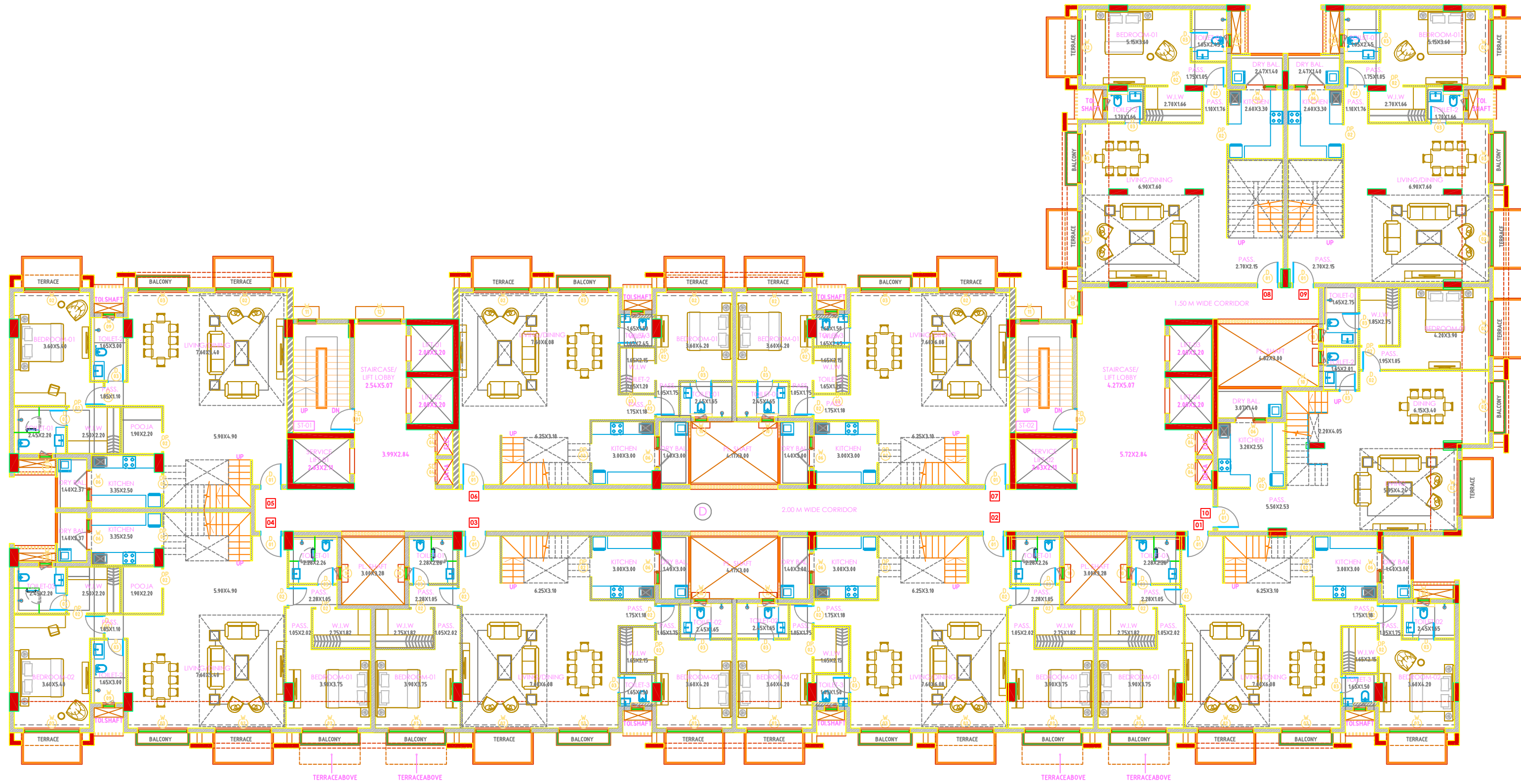
FIFTH FLOOR PLAN
